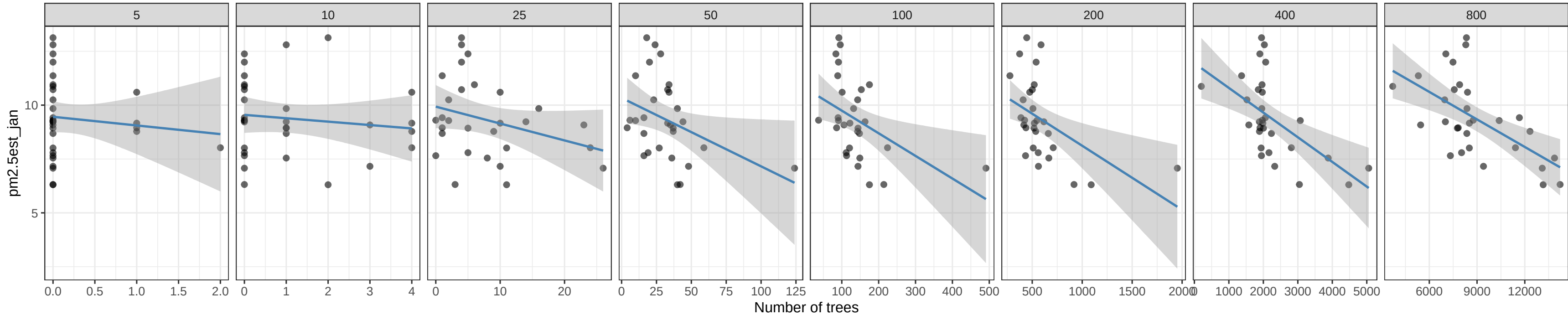
pm2.5est_jan vs Number of trees by buffer radius
